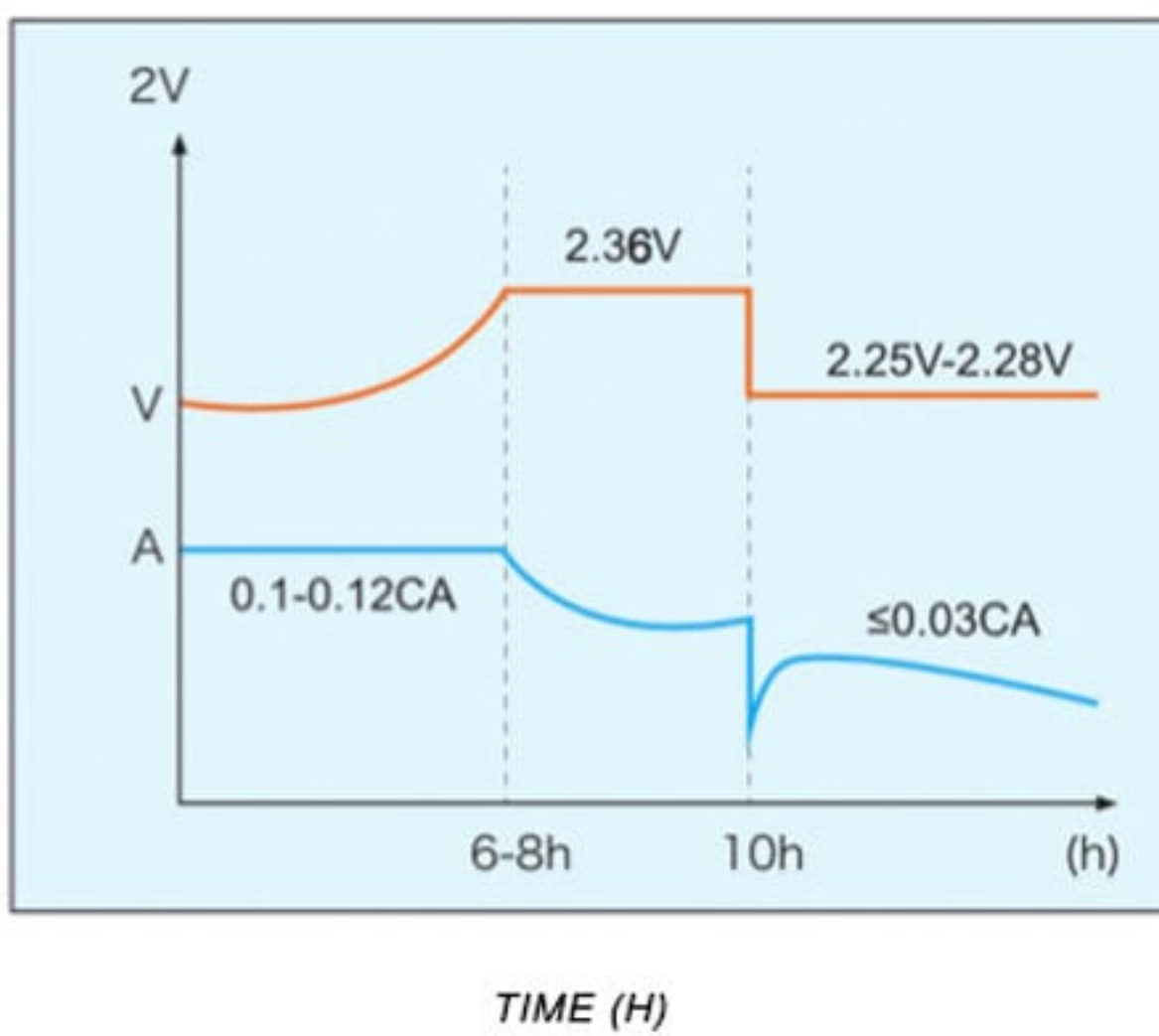
BATTERY CHARGE CURVE AT 25°C
