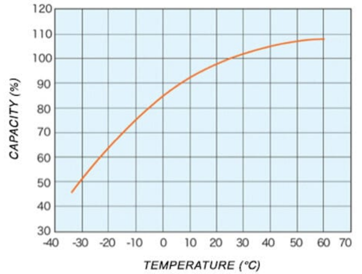
BATTERY CAPACITY VS. TEMPERATURE ENVIRONMENT
