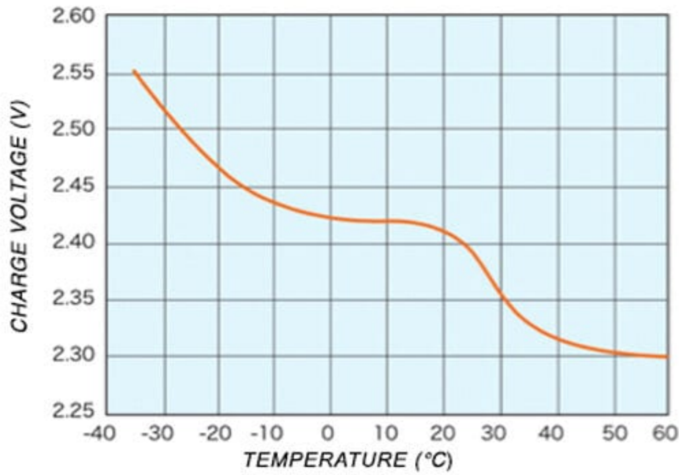
BATTERY CHARGE VOLTAGE VS. TEMPERATURE
