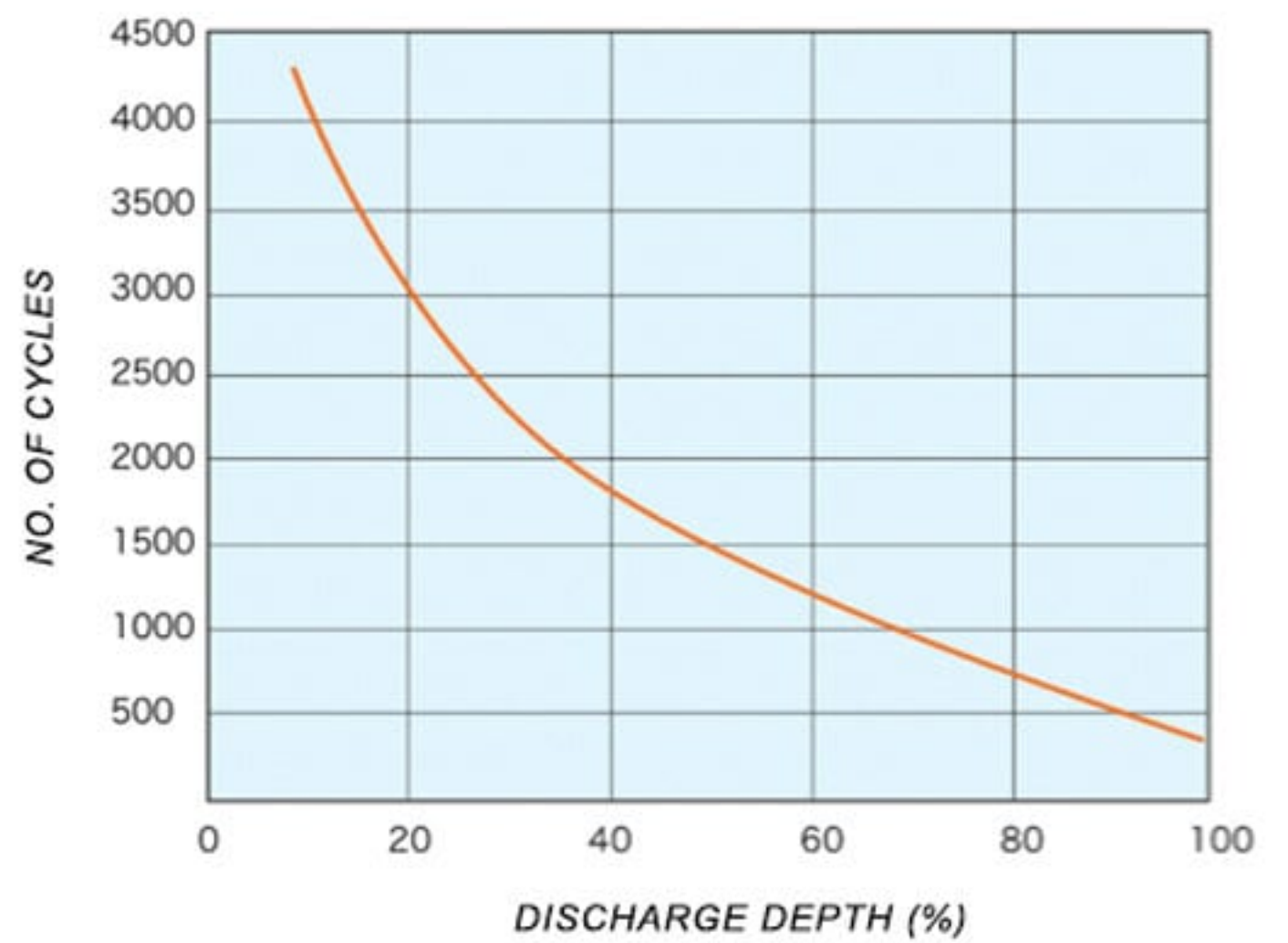
BATTERY DISCHARGE DEPTH VS. CYCLE TIME RELATION AT 25°C
