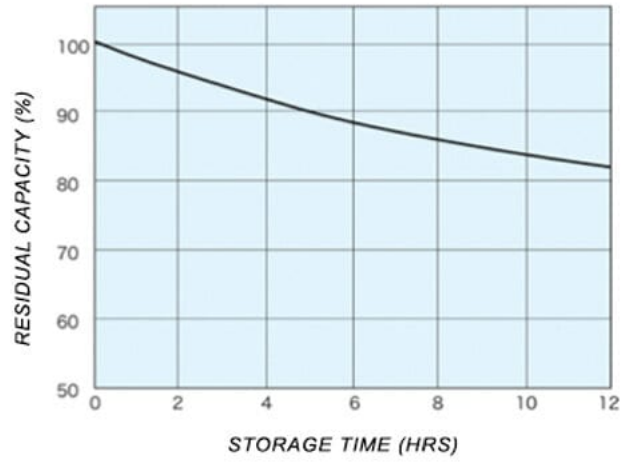
BATTERY SELF-DISCHARGE DURING STORAGE AT 25°C
