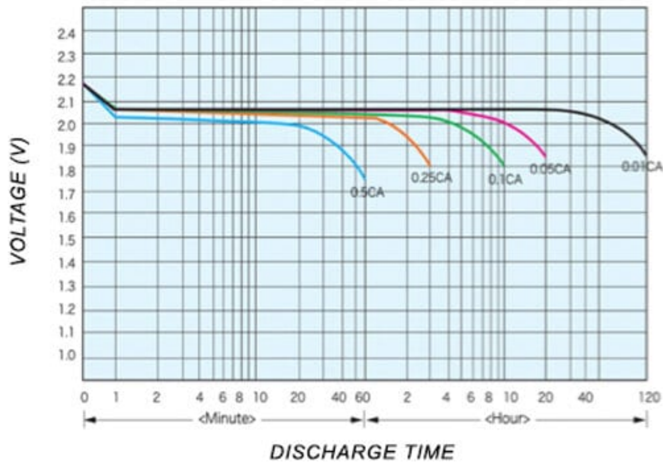
BATTERY DISCHARGE CURVE AT 25°C
